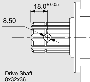
Drive Shaft
