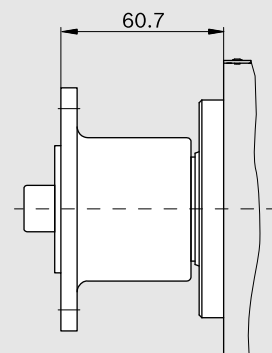
Coupling Flange
